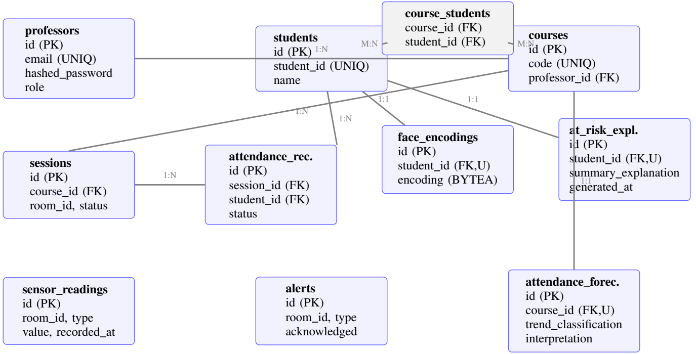
Fig. 8. Entity-Relationship Diagram.
