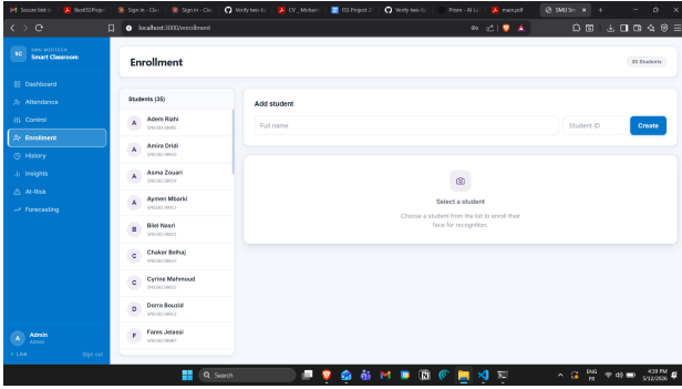
Fig. 14. Enrollment page.
