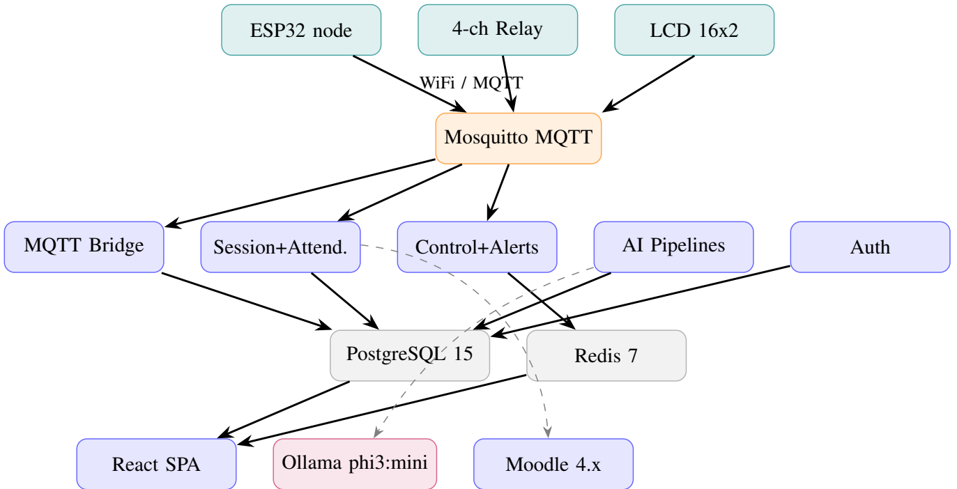
Fig. 2. Full system layered architecture diagram.
