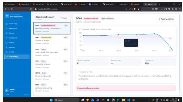
Fig. 13. Forecasting page.
